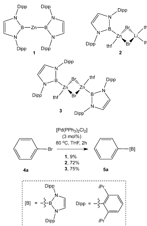
Figure 1. Borylzinc compounds employed in this work and their application in bromobenzene borylation chemistry.
